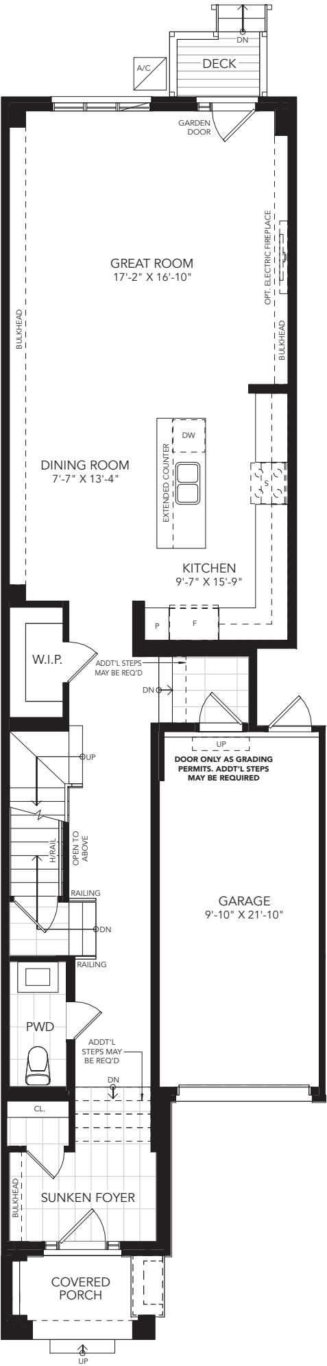
GROUND FLOOR PLAN A
