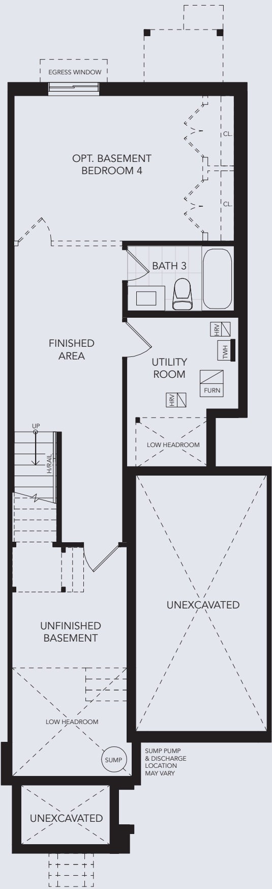
OPTIONAL FINISHED BASEMENT PLAN WITH OPTIONAL 4TH BEDROOM
